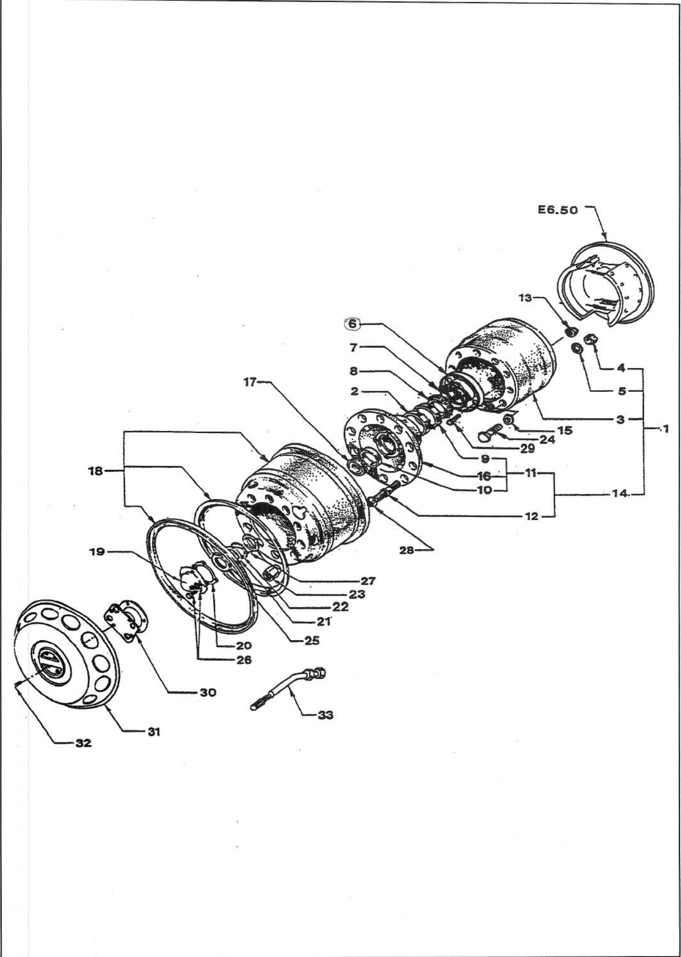
TEKERLEK DONANIMI - ÖN DINGİL WHEEL INSTALLATION - FRONT AXLE
